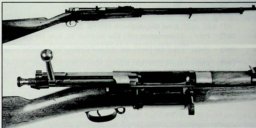
8 mm Krag-Jørgensen Rifle No. 71/1890
