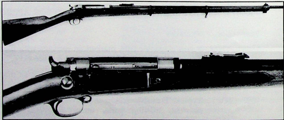
8 MM Krag-Jørgensen Rifle No. 61/1888
