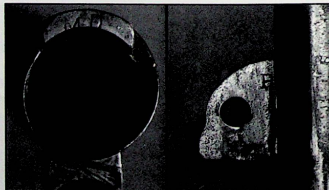
This M1911 barrel bears the mark MD above breech, possibly indicating it is one of those "austempered" as part of Springfield's Manufacturing Development Program No. 1 (see pg. 60-7). Only other mark is the usual small "P" proof marking (shown on right). Specimen courtesy Dr. Zachery Leiner.
