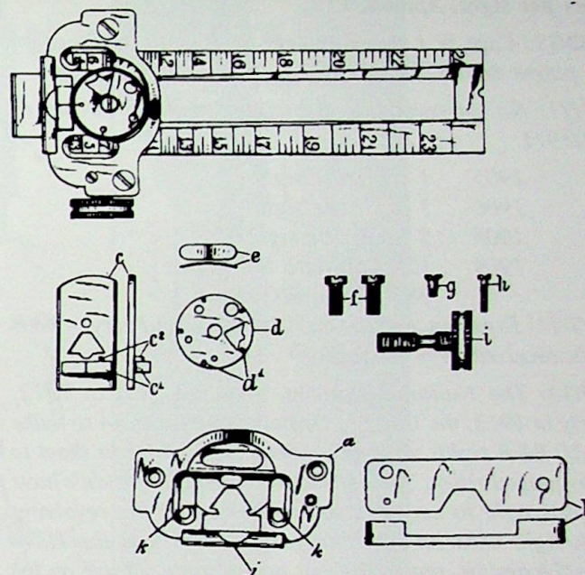
Drawing of Bassell & Blenkner sight, from NA RG 156 E 28 F 39019-52 5/28/08. Note binding screw, lack of elevation screw. The sight disk must be depressed on its top side in order to rotate it.
