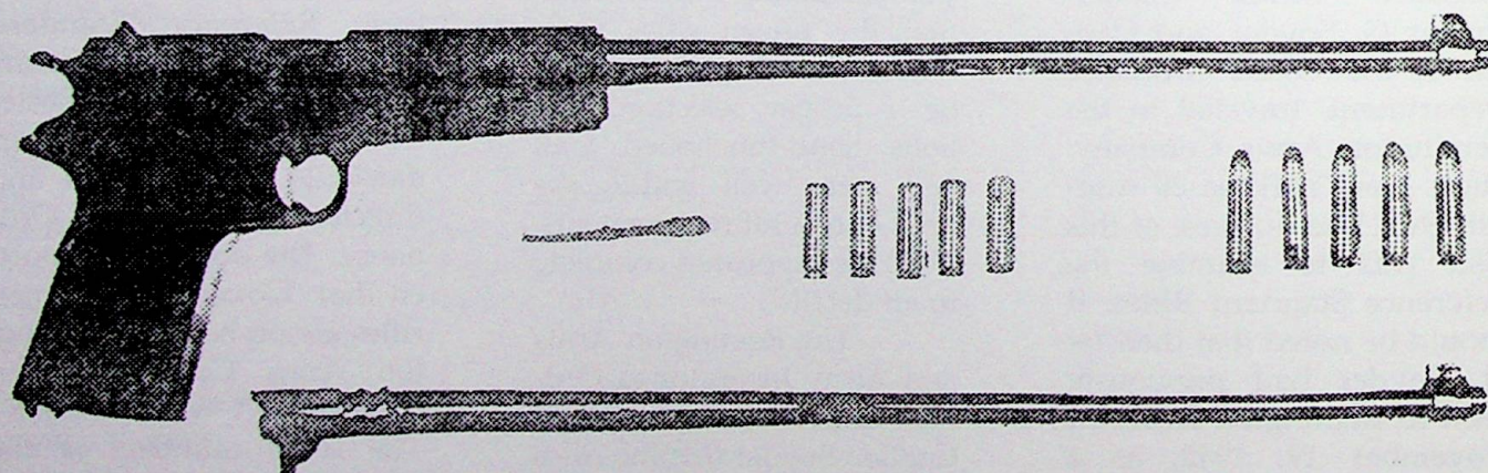
Proposed Survival Weapon: Carbine Pistol, Cal. .30 M1 (M1911A1 pistol adapted to use an M1 Carbine barrel chambered & bored for shot cartridges). From NA RG 338 Panama.
