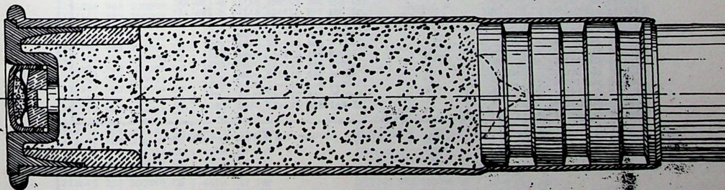
Morse Sliding-base Cartridge for Service Rifle
