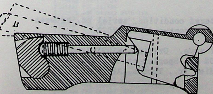
Buffington Firing Mechanism of Jan., 1883
