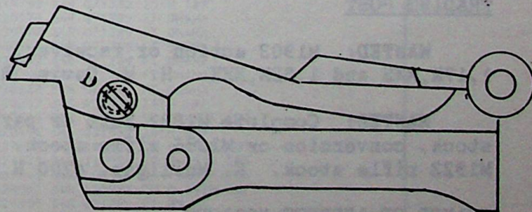
Buffington Firing Mechanism of Jan., 1883
